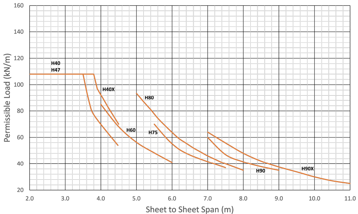
H Series - Permissible Load Chart
